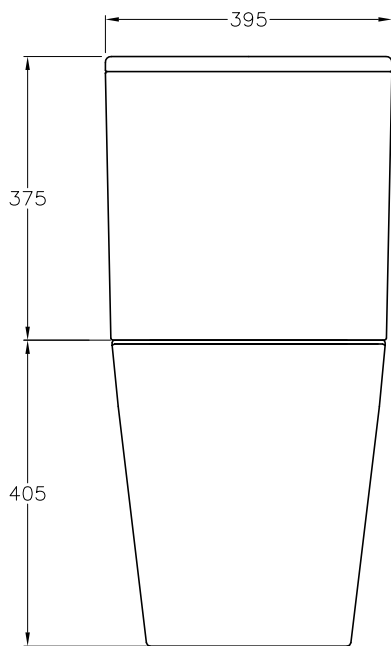
FRONT ELEVATION
